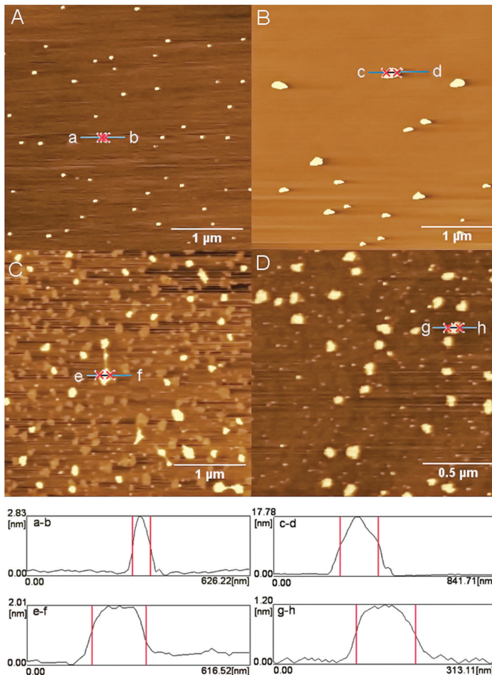
Fig. 9 Typical images of PBR322 DNA condensates in PEG-6000 solution (30% w/v) at varying \text{MgCl}_2 concentrations. From (A to D), the \text{MgCl}_2 concentrations are 0.1, 5, 300 and 500 mM. The corresponding typical profile measurements are shown in the bottom part of the figure.
