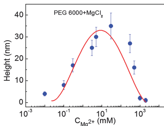
Fig. 7 The statistical height of the DNA-PEG complexes as a function of \text{MgCl}_2 concentration ( \sim 0.001 – 2000 mM) in the PEG-6000 solution (30% w/v). The error bars represent the standard deviation of the average of ten measurements. The data were fitted using a polynomial function.
