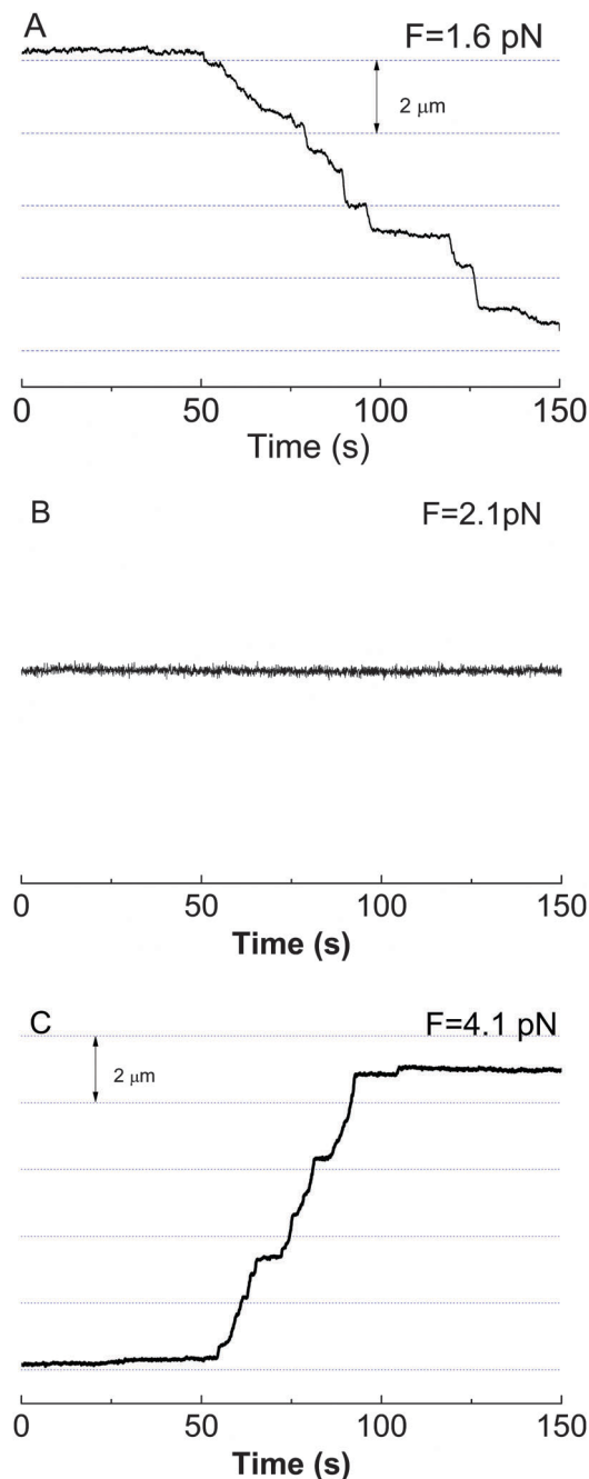
Fig. 11 Some representative curves in MT measurements under different constant forces. The loaded solution is PEG 6000 + 140 mM NaCl. F is the exerted force, -\Delta g is the condensation free energy per unit DNA length. (A) F < -\Delta g ; (B) F \sim -\Delta g ; (C) F > -\Delta g .
