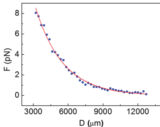
Fig. 3 Calibration of the F - D relationship.
