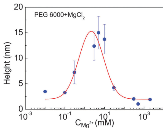
Fig. 10 The statistical height of the PBR322 DNA-PEG complexes as a function of \text{MgCl}_2 concentration ( \sim 0.01 – 2000 mM) in the PEG-6000 solution (30% w/v). The error bars represent the standard deviation of the average of ten measurements.
