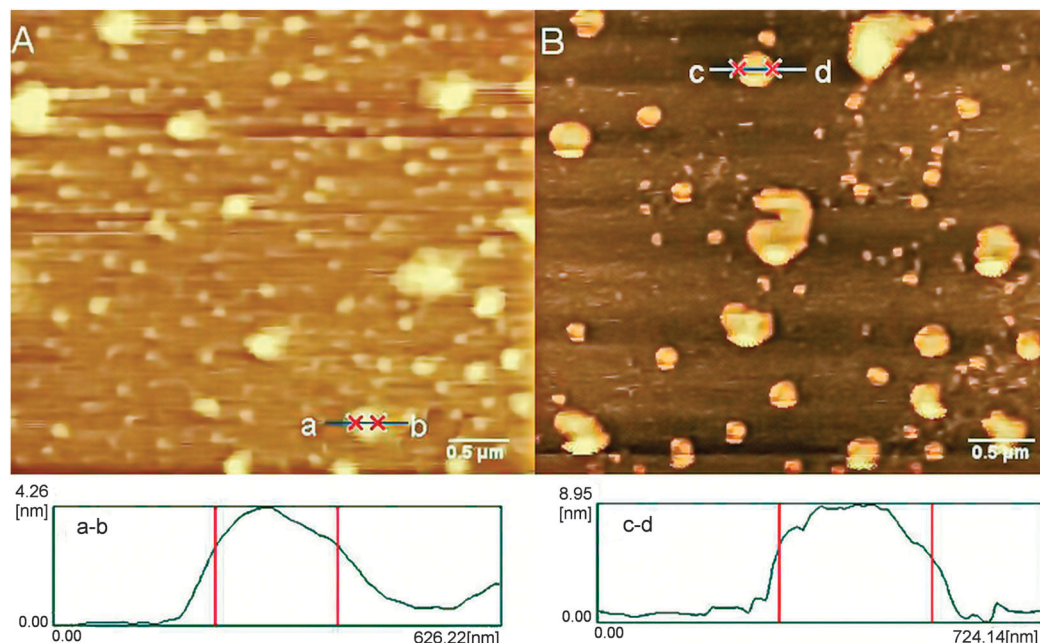
Fig. 8 Typical images of the PEG 600-induced DNA complexes under different salt conditions. (A) 800 mM NaCl; (B) 3 mM MgCl 2 . The heights of the measured complexes in (A and B) are ~4 and 9 nm, respectively.
