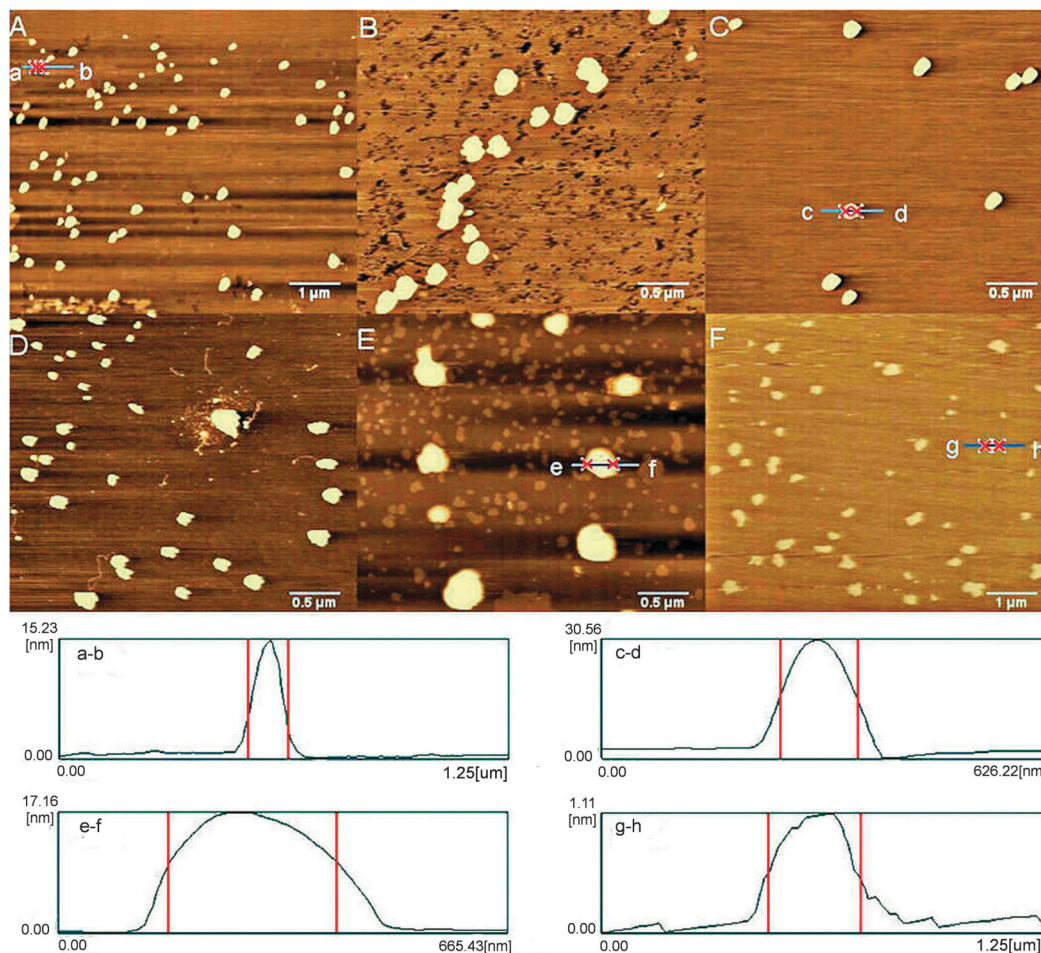
Fig. 6 Typical images of DNA condensates in PEG-6000 solution (30% w/v) at varying \text{MgCl}_2 concentrations. From (A to F), the \text{MgCl}_2 concentrations are 0.01, 3, 30, 300, 500, and 1000 mM. The corresponding typical profile measurements are shown in the bottom part of the figure.
